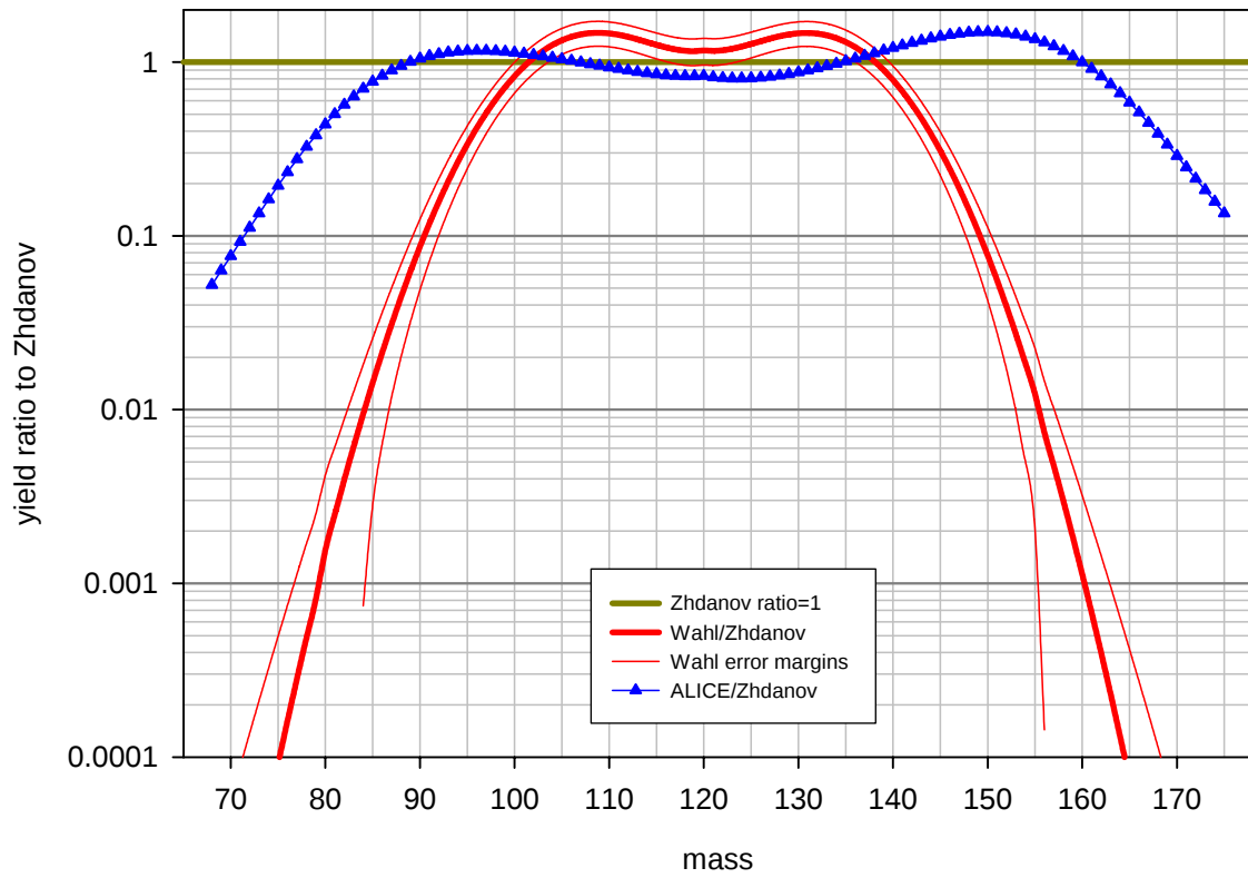
Benchmark B: ^{244}\text{Cm} at 100 MeV, pre-neutron emission yield ratio to Zhdanov's data
